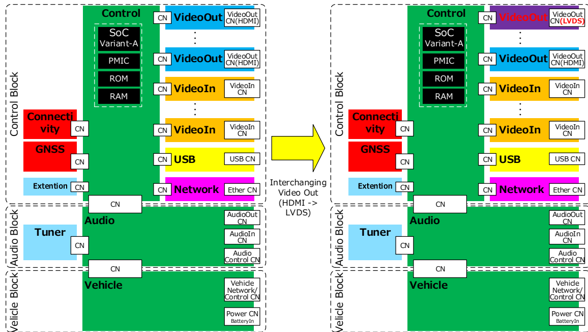
Figure 13 Interchanging Video Out (HDMI -> LVDS)
