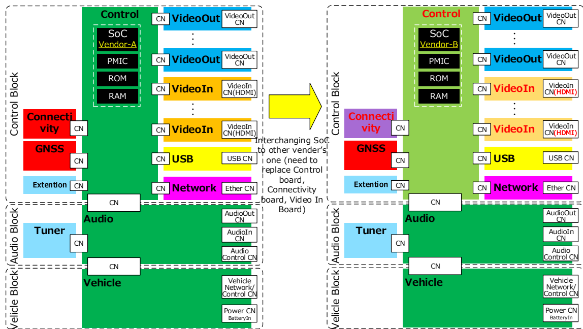
Figure 14 Interchanging SoC to other vendor's one
