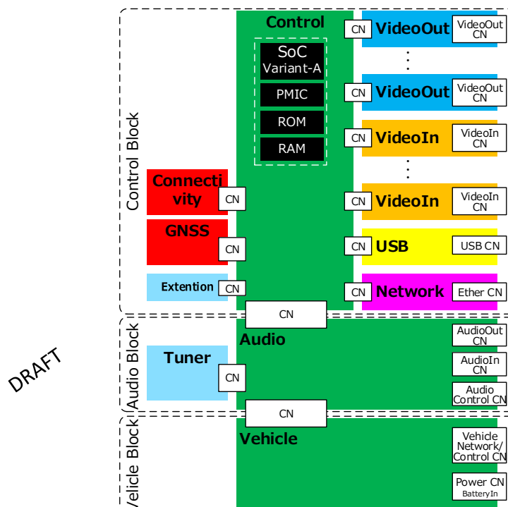
Figure 11 Selectable and Interchangeable architecture
