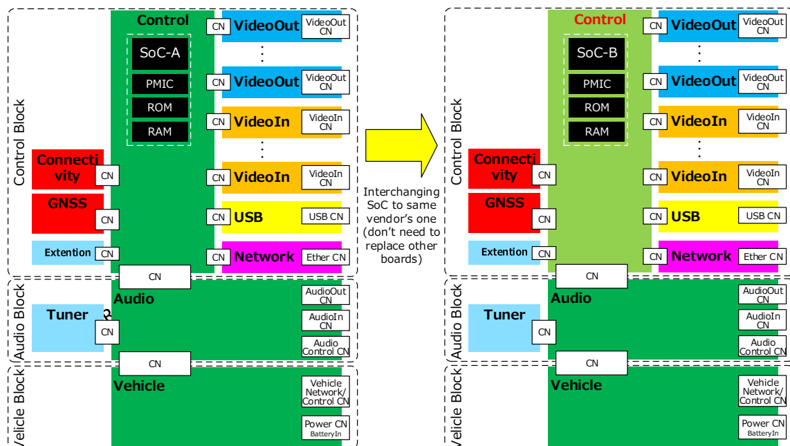
Figure 12 Interchanging SoC to same vendor's one
