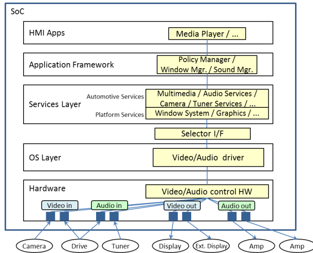
Figure 8 <T.B.D.> An image of Selector implementation (Connected to SoC)
