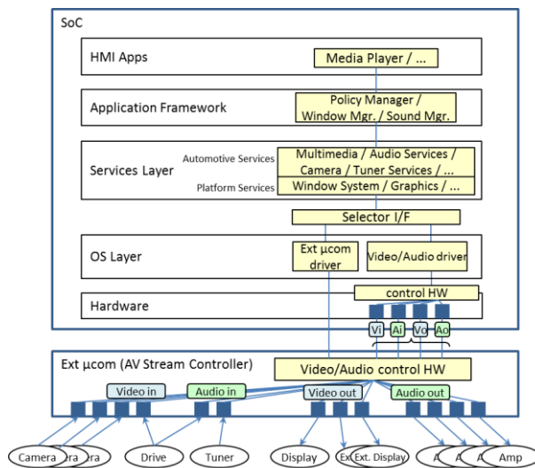
Figure 9 <T.B.D.> An image of Selector implementation (Connected to AV Stream Controller)
